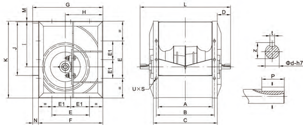
BND/BAD-GM Dimension
