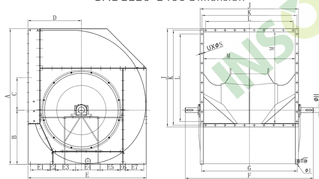
BAD1120-1400 Dimension
