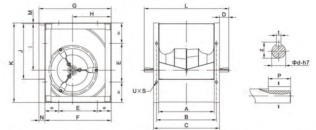
BND/BAD-K Dimension
