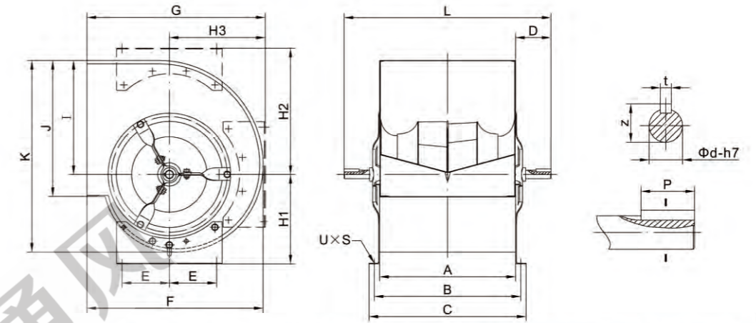
BND/BAD-D Dimension
